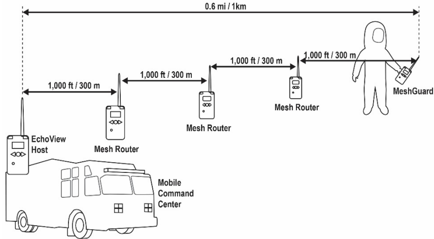
Range extension with Mesh Routers.
