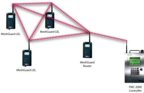
MeshGuard LEL network with FMC-2000 controller
