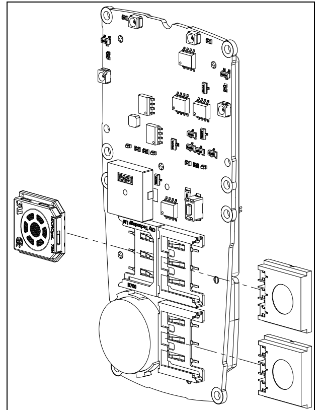
Figure 11. Sensor Positioning
