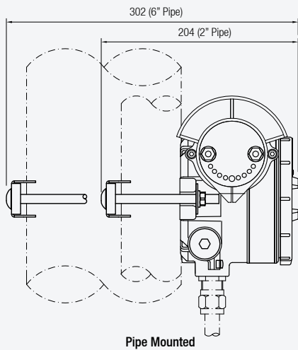
Pipe Mounted
